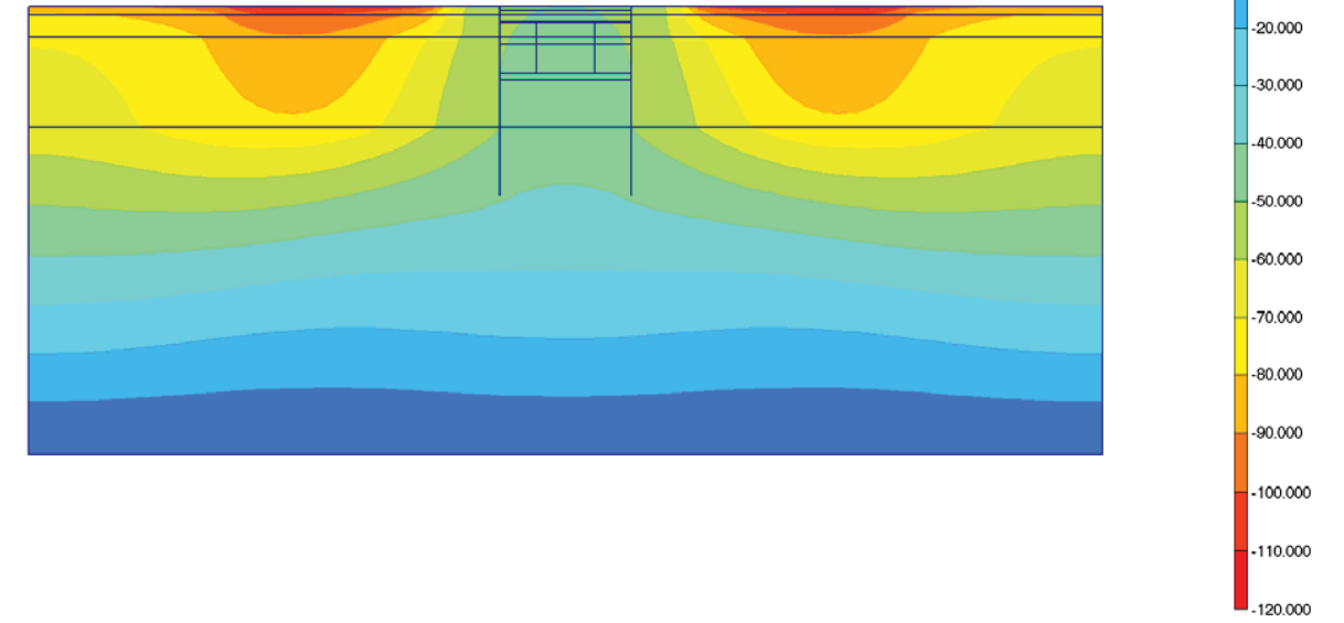
Fig. 13 Plot of vertical displacements (shadings) - step no: 4 - ( phase: 1 )
